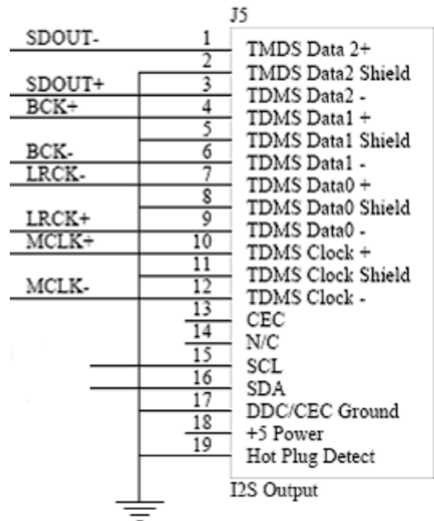
GLD 1.0 I2S Interface
